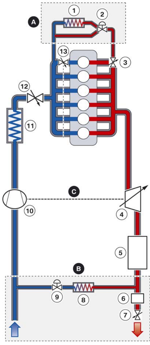
Schematic diagram of high and low-pressure exhaust-gas recirculation for B57 engine in the G30
