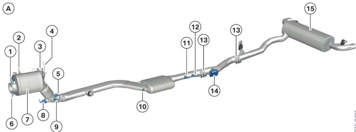
BMW G30 B57 engine exhaust systems
