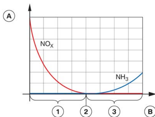
Nitrogen oxide and ammonia emissions diagram for the SCR system
