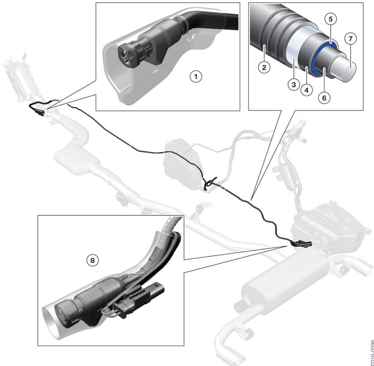
SCR 3, metering line
