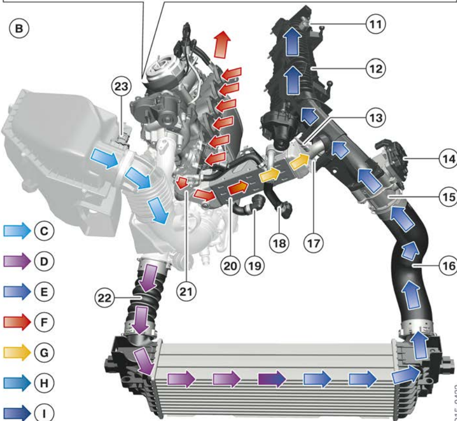
Overview of high and low pressure EGR for the B57 engine
