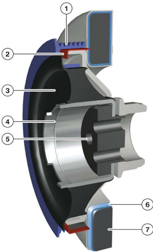
Torsional vibration damper, B57 engine
