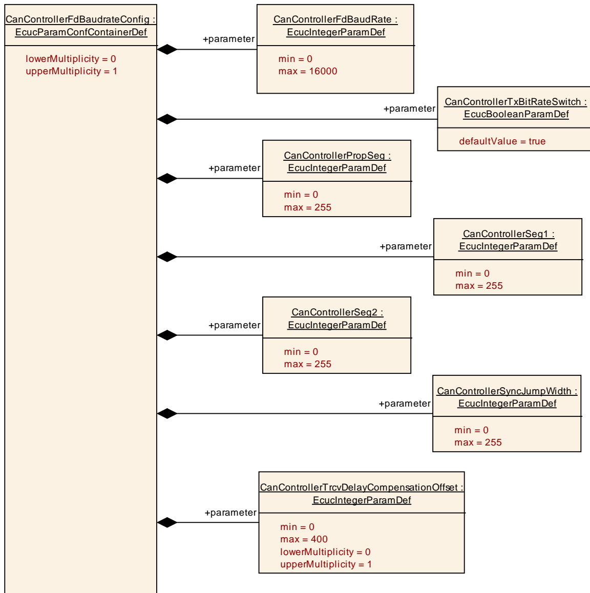
Figure 10-5: CanControllerFdBaudrateConfig
